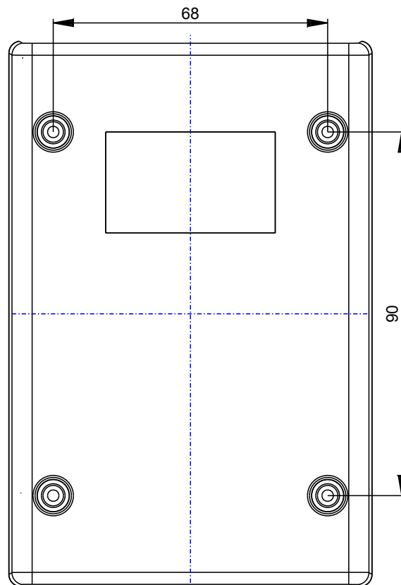
Option -M3: 4x M3-thread
